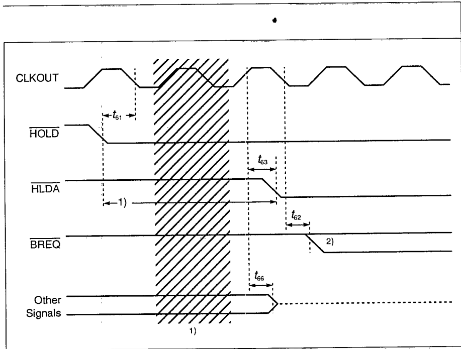
Figure 15 External Bus Arbitration, Releasing the Bus
