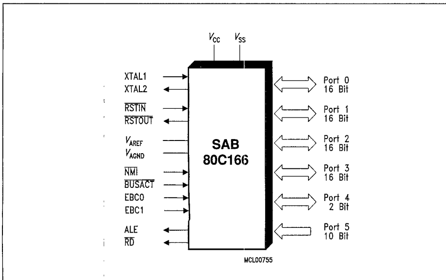
Figure 1 Logic Symbol
