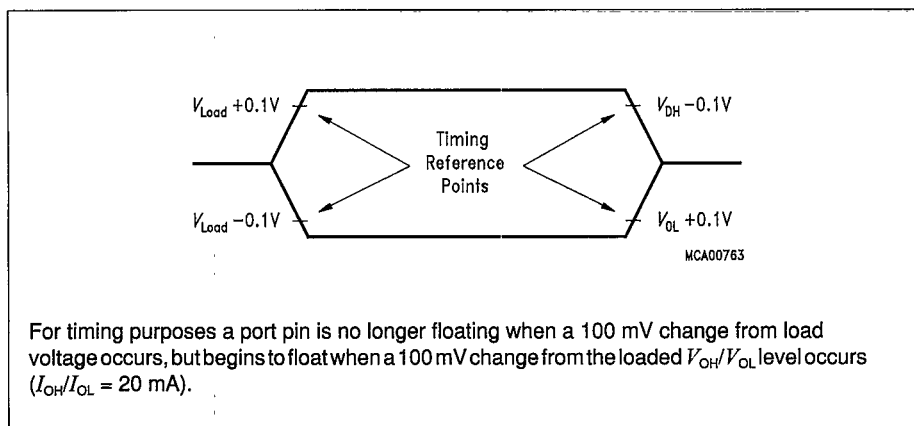
Figure 10 Float Waveforms
