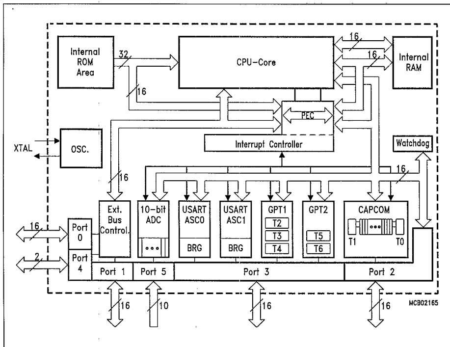
Figure 3 Block Diagram
