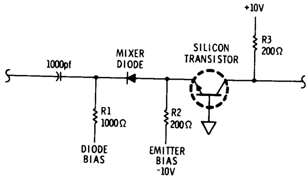
Figure 8-12. First Converter Assy, Simplified Schematic
