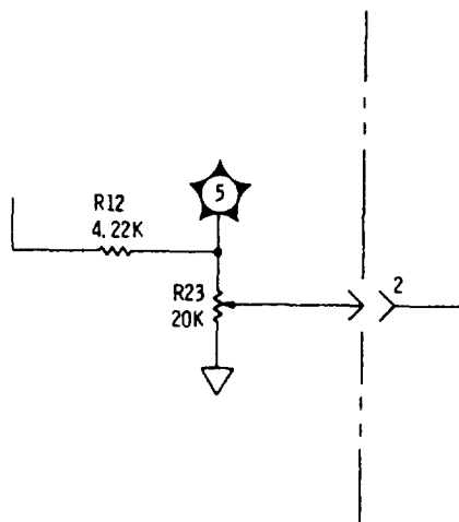
P/O Figure 8-38. Signal Identifier (CHANGE 4)
