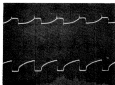
A A9A1U1E Base Volts/Div: 2 Time/Div: 5 \mu sec B U1E Collector Volts/Div: 10 Time/Div: 5 \mu sec
