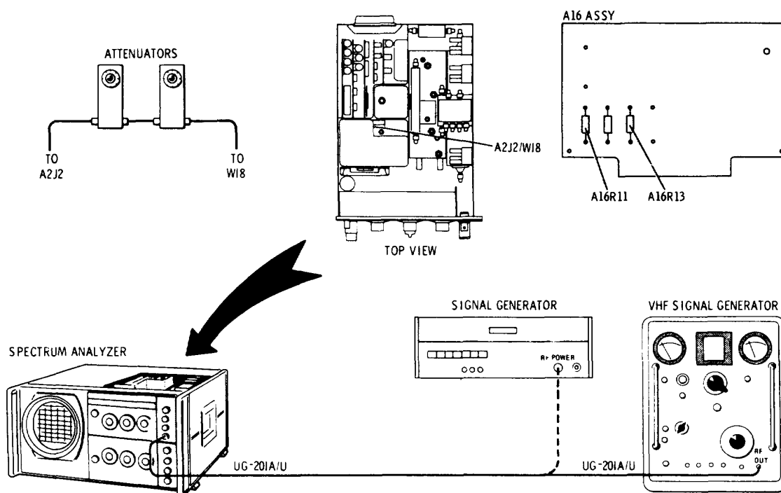
Figure 5-8. 50 MHz Amplifier Check and Adjustment Test Setup
