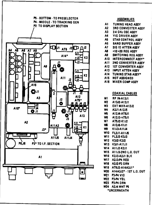
INTERNAL VIEWS
