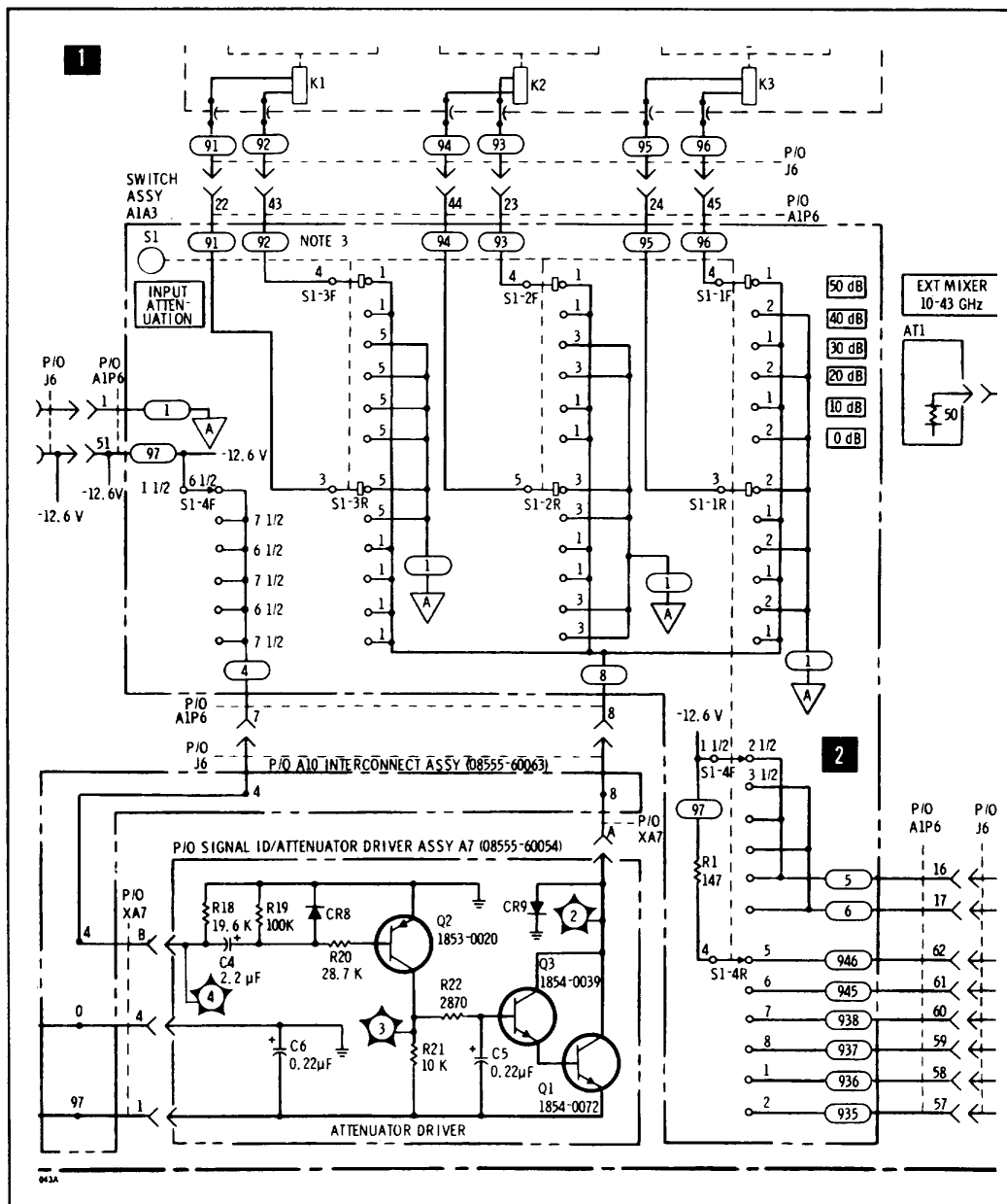
Figure 7-7. Partial Schematic of Figure 8-17 Showing A1P6 Pin Changes (P/O Change E)
