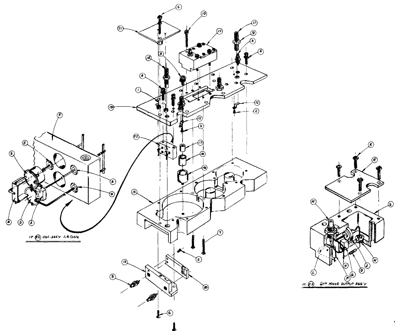
Figure 8-76. Second Converter Casting, Illustrated Parts Breakdown
