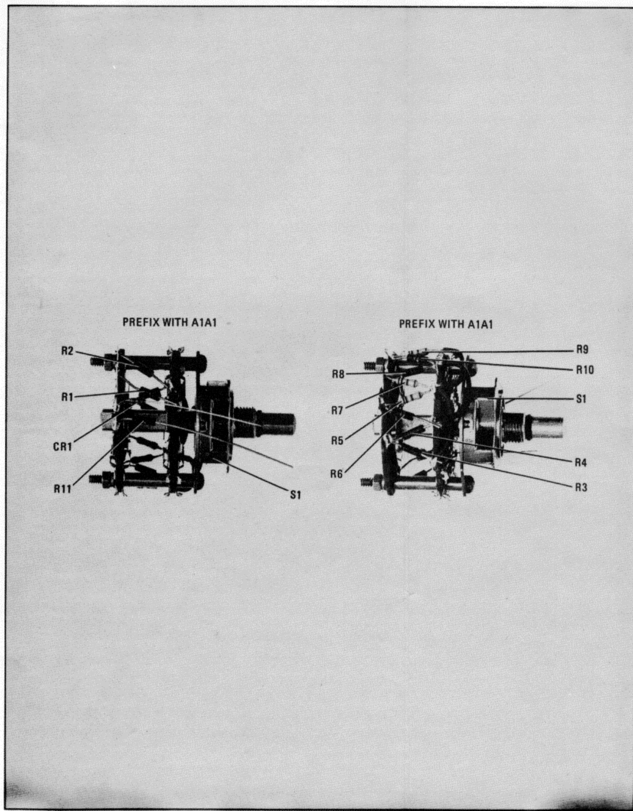
Figure 8-66. Bandwidth Switch Assembly A1A1
