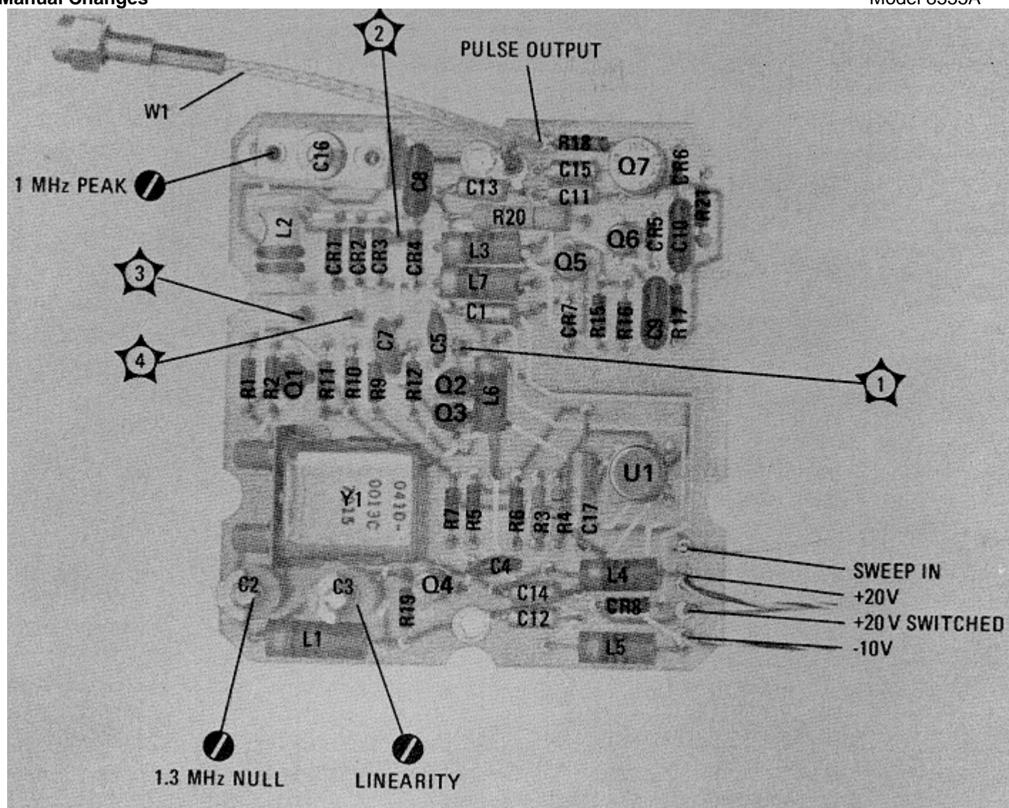
Figure 7-17. Tuning Stabilizer VCXO Assembly A14A2 (08555-60058), Figure 8-53 (Change Q)
