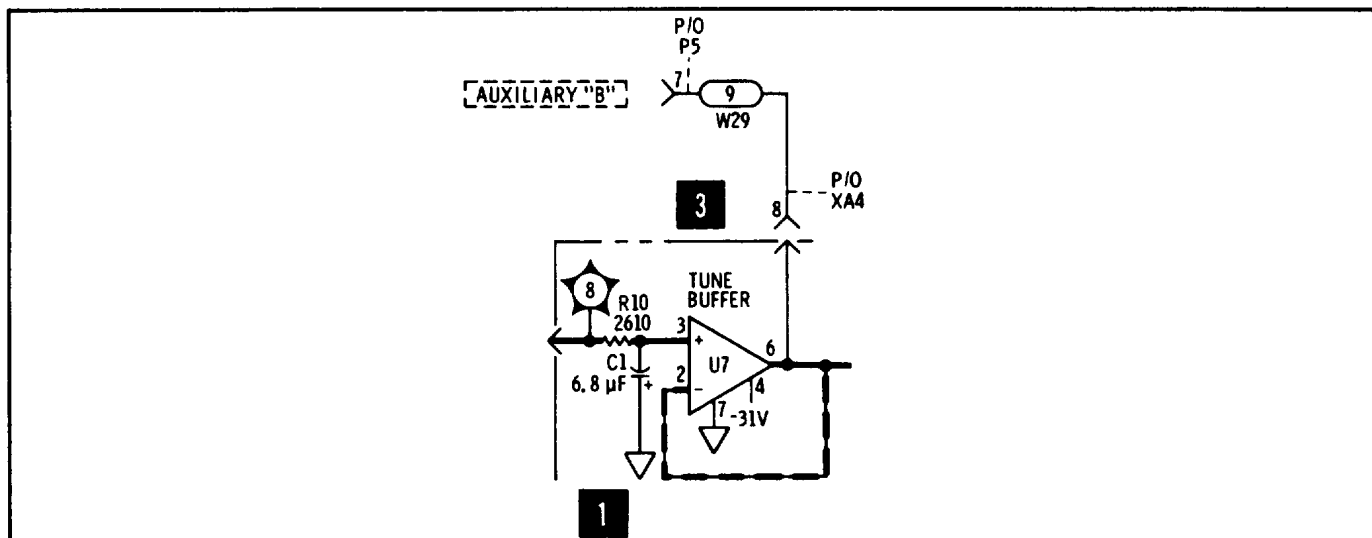
Figure 7-6. Partial Schematic of Figure 8-41 (P/O Change C)
