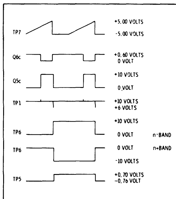
Figure 8-35. Signal Identifier Timing Diagram
