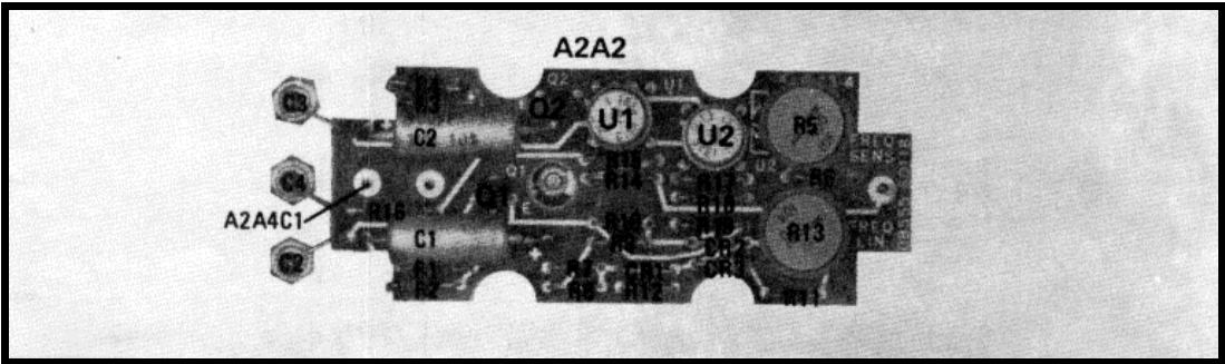
Figure 8-23. 500 MHz LO Drive Assembly A2A2
