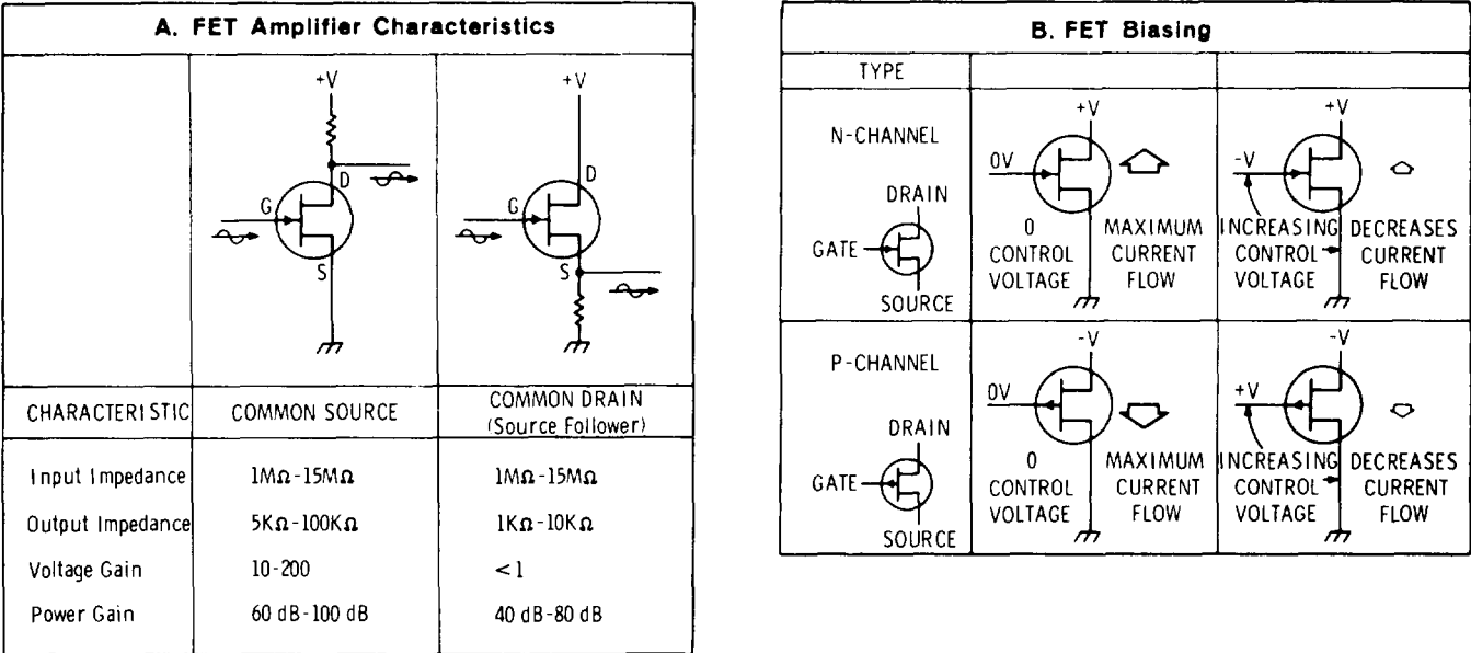
Figure 8-2. Field Effect Transistor Operation
