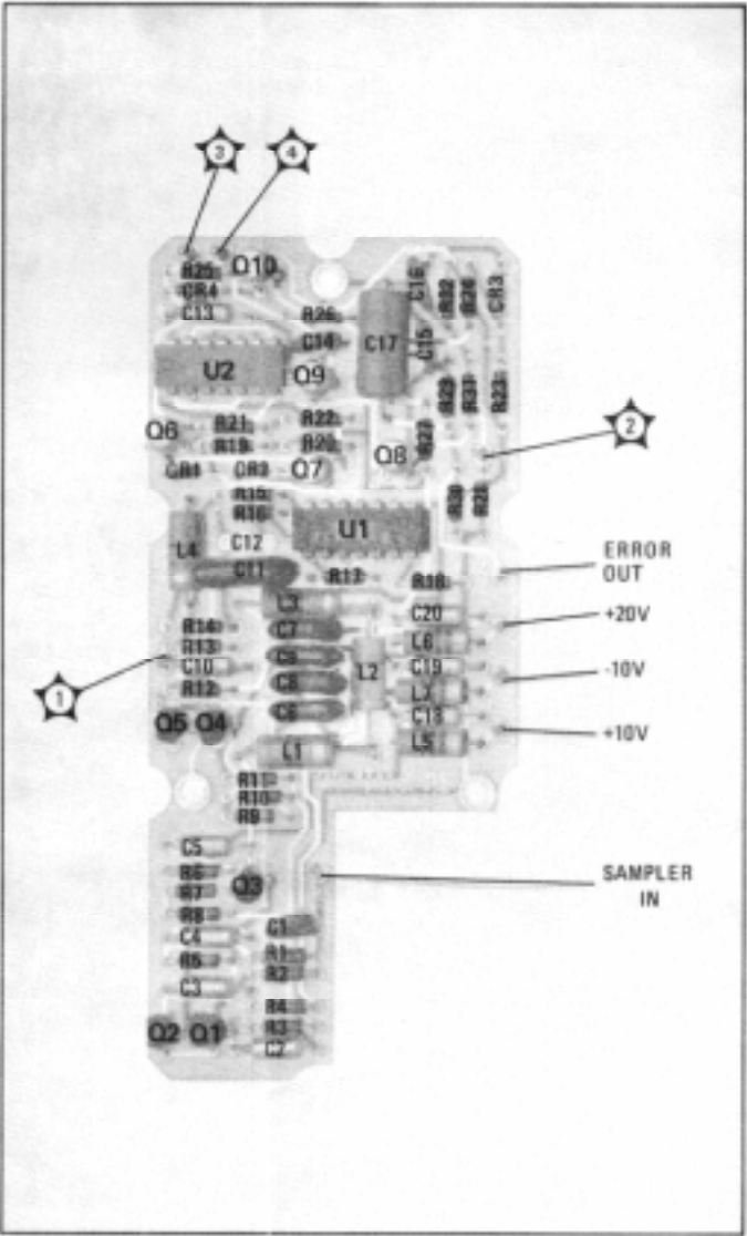
Figure 8-51. Discriminator assembly A14A1
