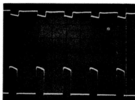
A A9A1Q1 Emitter Volts/Div: 10 Time/Div: \mu 5 sec B A9A1Q2 Collector Volts/Div: 50 Time/Div: 5 \mu sec
