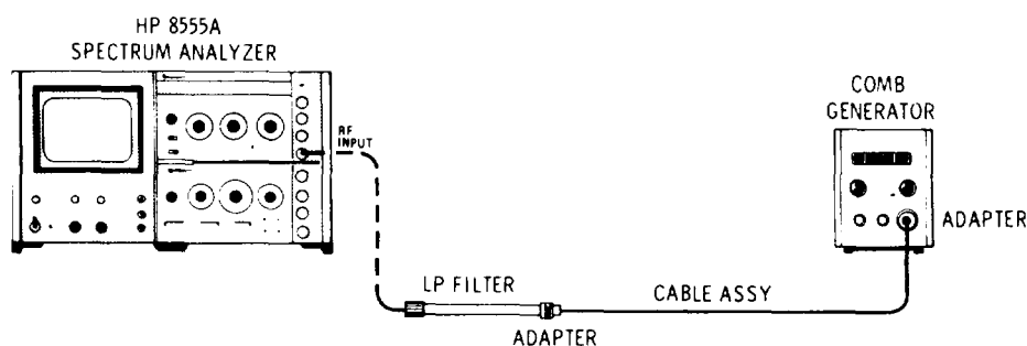
Figure 4-9. Residual FM Test Setup
