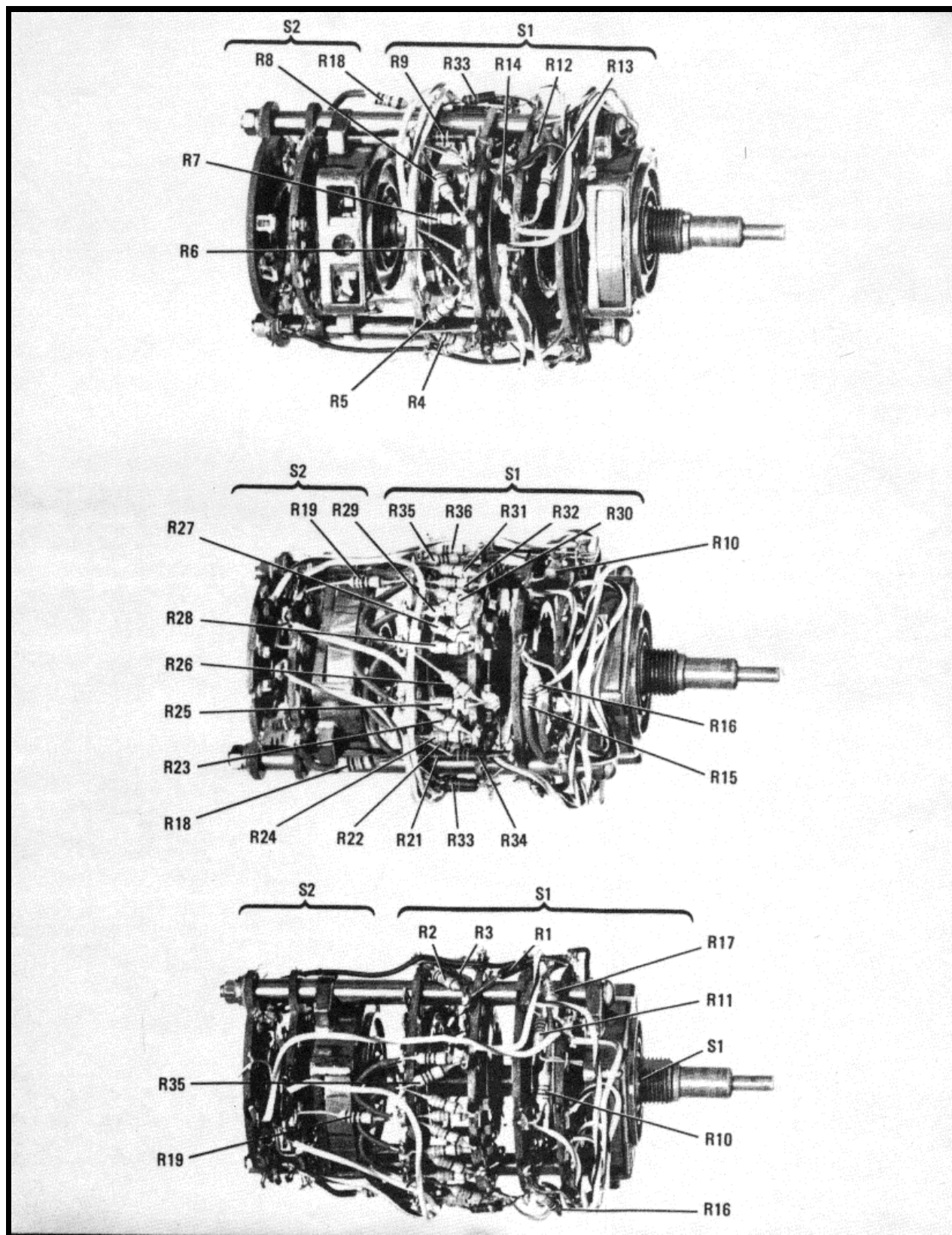
Figure 8-63. Scan Width Switch Assembly A1A2
