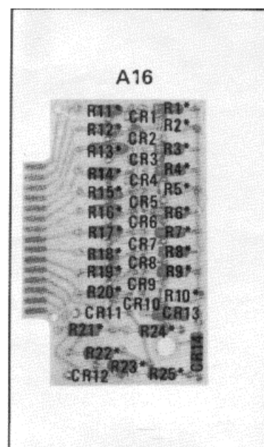
Figure 8-32. Input Mixer Network A16
