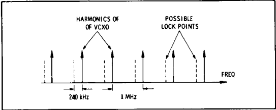
Figure 8-47. VCXO Harmonics and Lock Points
