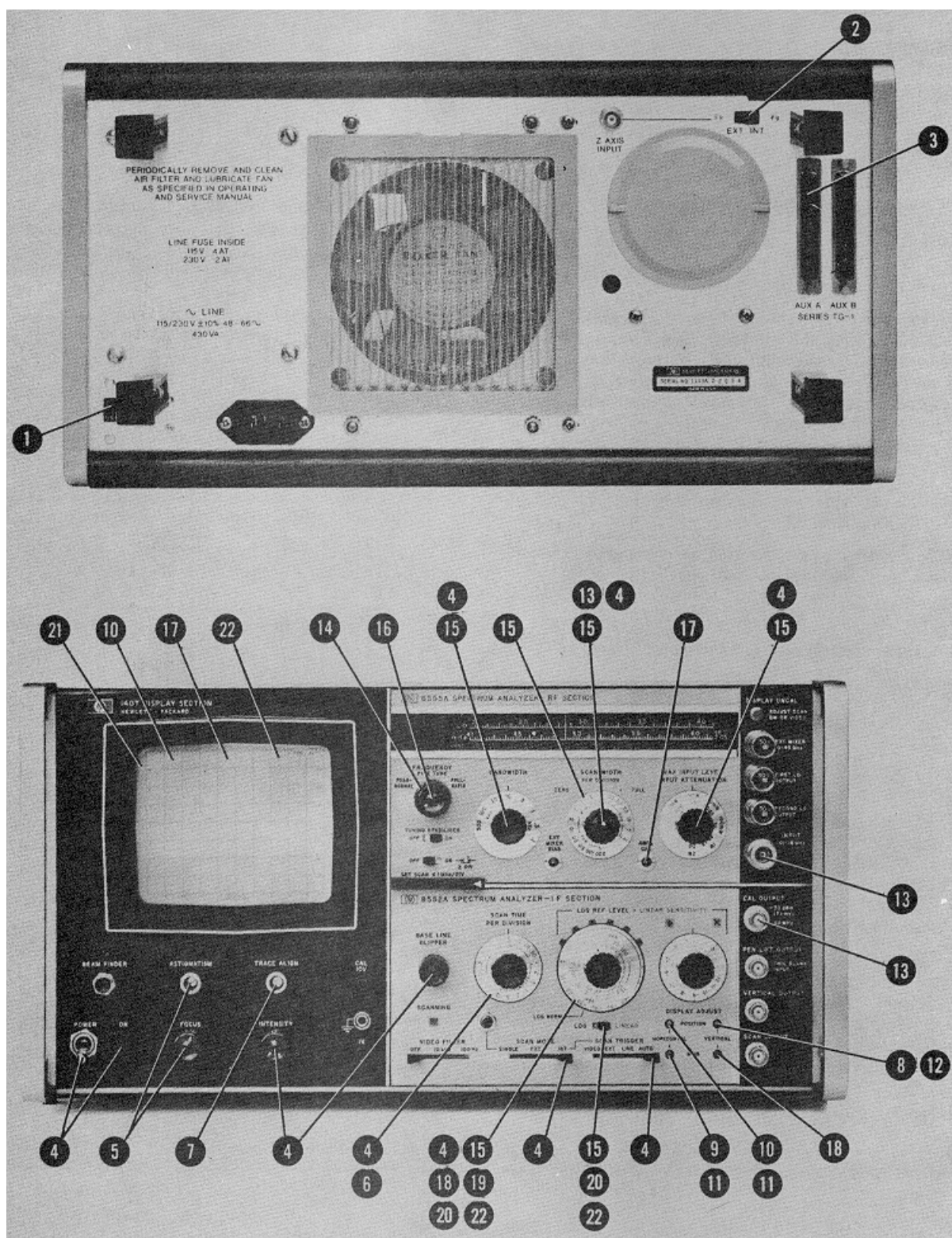
Figure 3-3. Operational Adjustments
